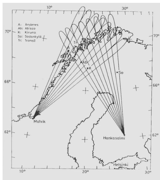
Fig. 6: STARE antenna beam pattern, the field of view covered a geomagnetic latitude range from 65 ° to 70°.
