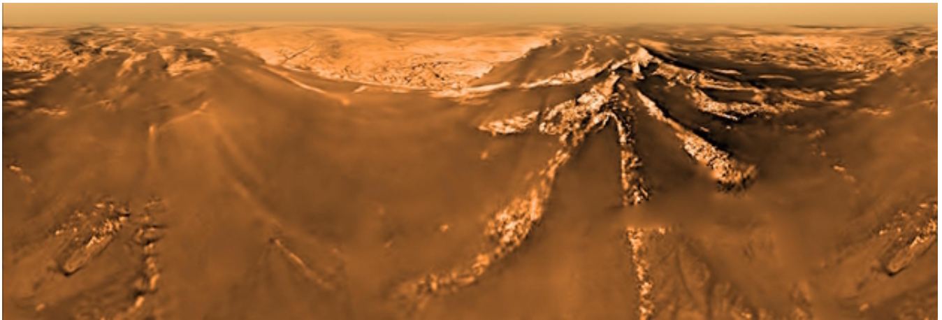
Fig. 9: Surface of TITAN photographed with DISR DESCENT IMAGER on Huygens on 14. July 2005 from an altitude of 2 km (Source: Lunar and planetary Laboratory, University of Arizona, MPAe).
