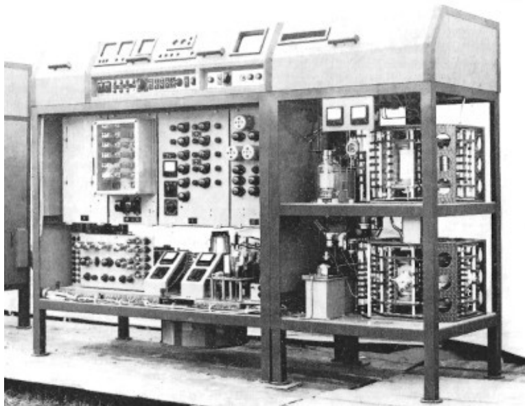
795 Fig. 3: Ionosonde from 1957 (Source: MPAe)
