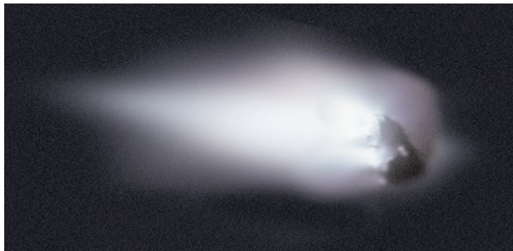
825 Fig. 12: Nucleus of Comet Halley photographed from a distance of 596 km on 14 March 1986 (Source: MP Ae).
