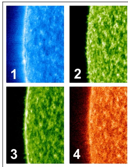
815 Fig. 10: East Limb Scan of the Sun with SUMER in four spectral lines, taken on 6 March 1996. 1: Ne VIII 780.324 Å (630 000 K), 2: O IV 790.20 Å (170 000 K), 3: C IV 1548.20 Å (1000 000 K), 4: Fe II 1563.79 Å (12 000 K). (Source: MPS, SUMER study #134)
