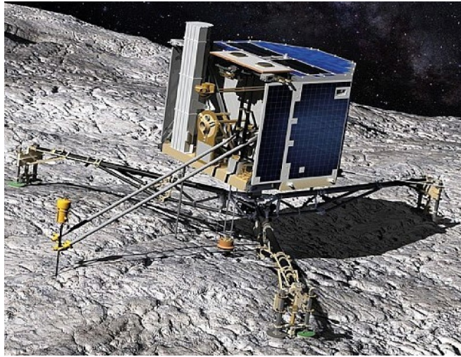
Fig. 13: The Lander Philae of the Rosetta project. It was anchored to the comet by screws at the end of the three shock absorbing legs and contained ten scientific instruments (source: DLR).
