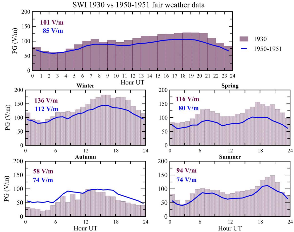
Fig. 3. Average diurnal variation of fair-weather (simple criteria: PG positive values, no thunderstorms and precipitation) electric potential gradient (PG) measured in Świder in 1930 (bars), and in 1950-1951 (solid line). Year-average variations are shown in the upper panel, and the seasonal curves are shown in the four panels below. Mean average values are displayed in the top left corner.
