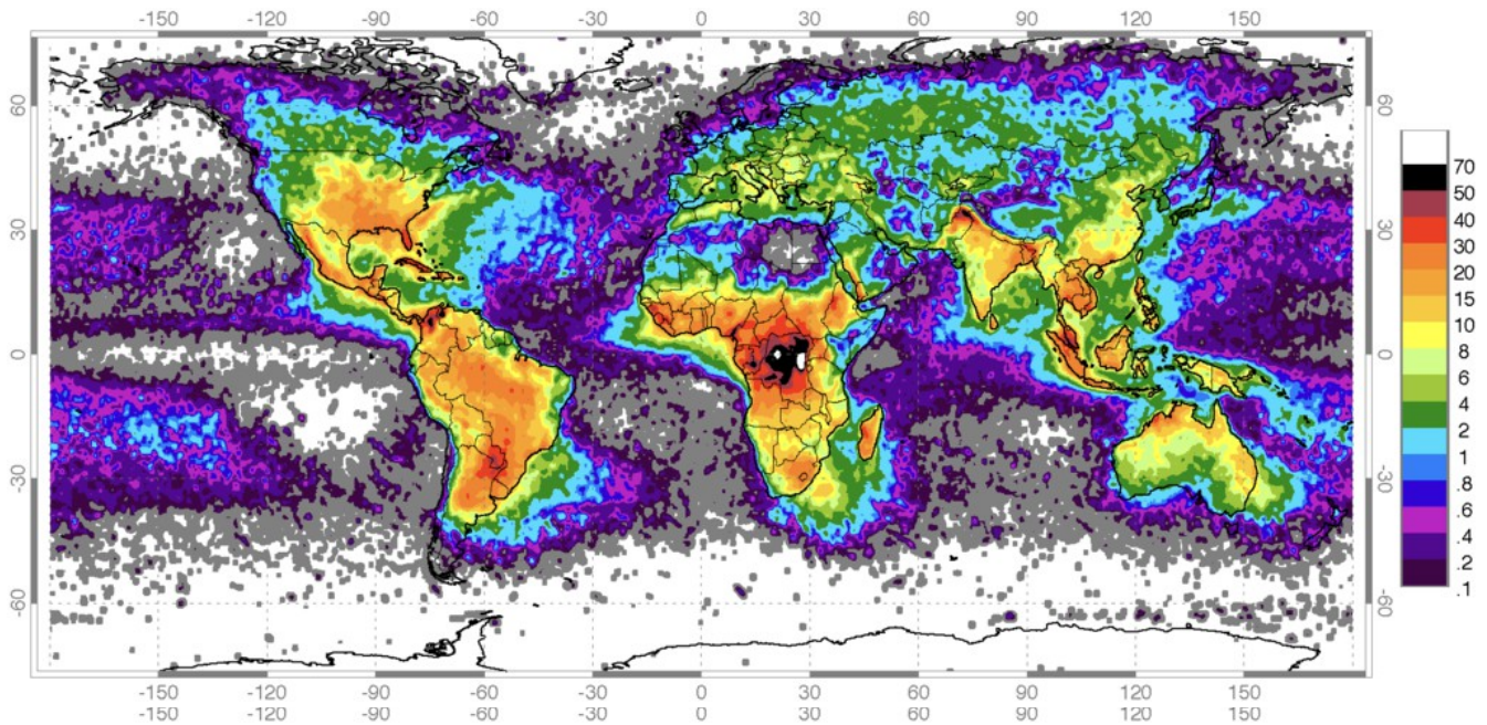
360 Fig. 4: Worldwide lightning strikes, data obtained from April 1995 to February 2003 from NASA's Optical Transient Detector. Public domain, WIKIMEDIA Commons.
