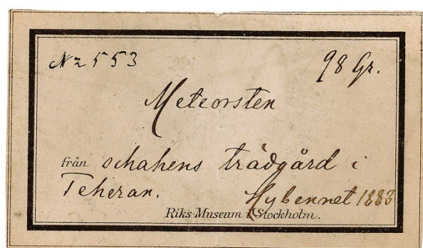
Figure 3. Original specimen label, Swedish Museum of Natural History, representing a part of one of the larger sample masses outside Iran. “Meteor stone from the gardens of the Shah in Tehran. Hybennet 1883”. Reproduced from original archival document.
