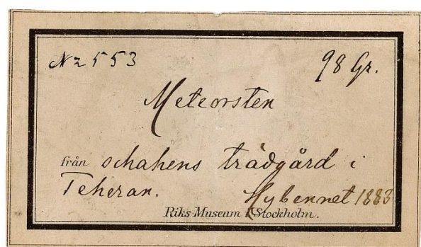
Figure 3. Original meteorite specimen label, Swedish Museum of Natural History, representing a part of one of the larger sample masses outside Iran. “Meteor stone from the gardens of the Shah in Tehran. Hybennet 1883”. Reproduced from original archival document.
