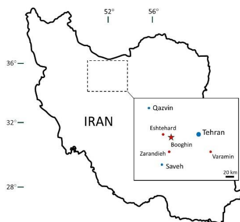
Figure 5. Map of Iran, with the key localities mentioned in the text. The meteorite likely fell near Booghin, located nearly 100 km from Varamin (Veramin). Drawing by authors.
