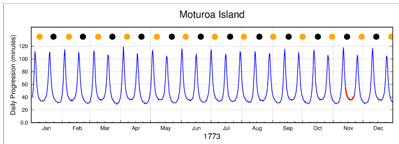
355 Figure 10. The predicted daily progression of high waters throughout 1773 at Moturoa Island; the portion in red corresponds to the period that Wales was making his observations.
