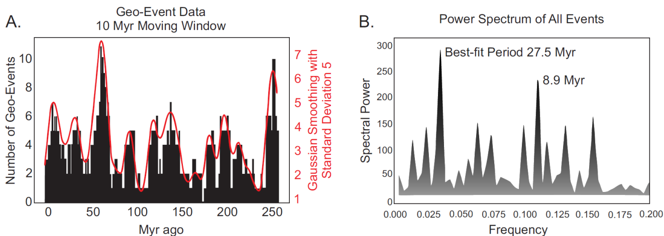
100 Figure 1. A - Analysis of the ages of 89 geologic events using a 10-Myr moving window centered every 0.5 Myr, with the number of occurrences that fall within the moving window computed at 1-Myr intervals. Ten clusters (peaks) are visible. In red, the Gaussian smoothing with a standard deviation of 5 Myr centered at every 0.1 Myr, with ten peaks. B - Fourier transform results show the highest peak in 27.5 Myr, and a strong secondary period occurs at 8.9 Myr (modified from Rampino et al., 2021).
