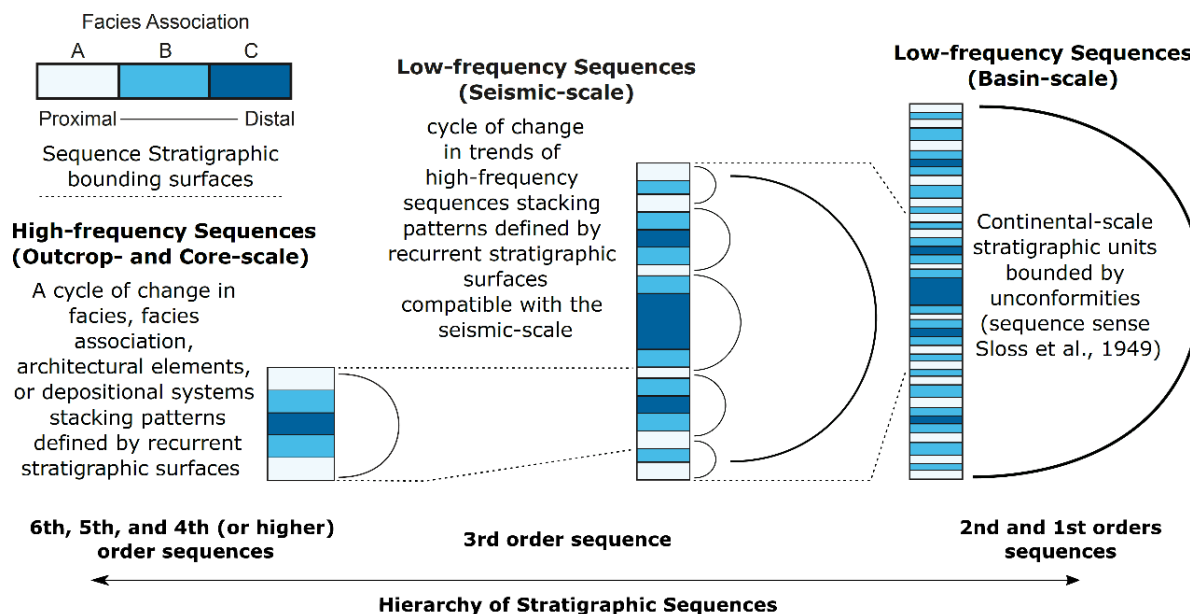
Figure 26. Hierarchical stratigraphic sequence framework (modified from Magalhães et al., 2020). High-frequency sequences (fourth or higher orders) are observed at outcrop- and core-scale. The vertical recurrence of high-frequency sequences composes the low-frequency sequences observed in seismic data (third-order). First- and second-order low-frequency sequences occur at basin-scale predominantly limited by unconformities, as proposed by Sloss et al. (1949).
