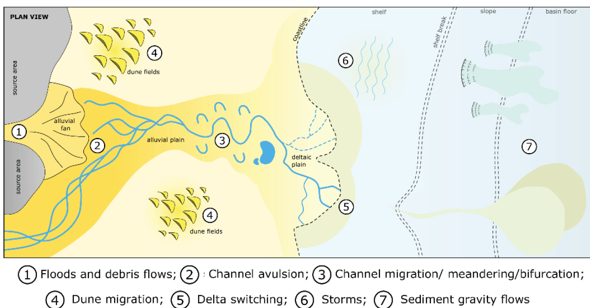
500 Figure 16. Schematic illustration with some autogenic controls on sedimentation in different environments.
