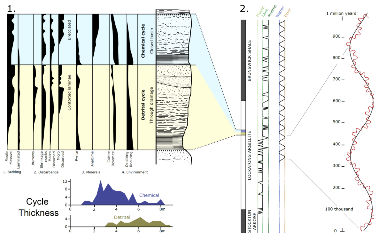
665 Figure 27. Cyclic lacustrine sedimentation of the Upper Triassic Lockatong Formation (modified from Van Houten,1964): 1. Model of detrital and chemical short cycles; 2. Generalized stratigraphic section of Lockatong Formation and adjacent units. The columns show the alternating geographic environments and the long climatic cycles of wetter and drier phases. An age model is presented based on two long climatic cycles, with intermediate and short cycles associated.
