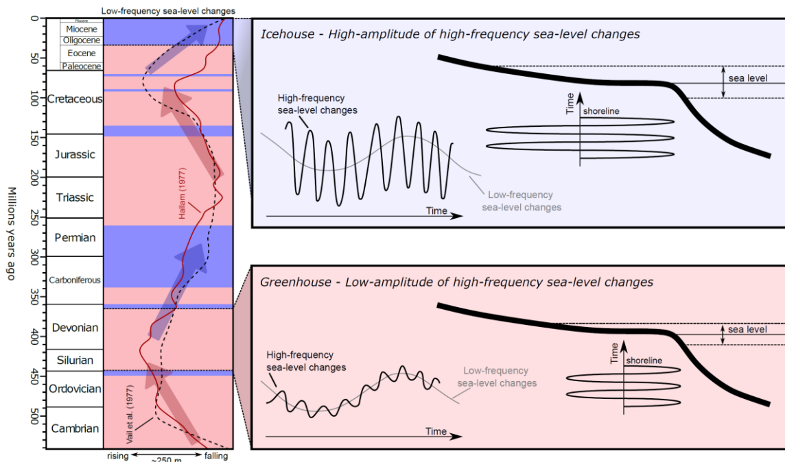
230 Figure 5. Changing frequencies and amplitudes of eustasy. Sea-level curves, according to Vail et al. (1977) and Hallam (1977). In icehouse periods (in blue), these cycles have a high amplitude, mainly due to the effects of glacioeustasy. Eustatic oscillations have lower amplitude in greenhouse periods (in light red) since there is no significant glacial effect (modified from Wilson, 1998; Séranne, 1999; Montañez et al., 2011).
