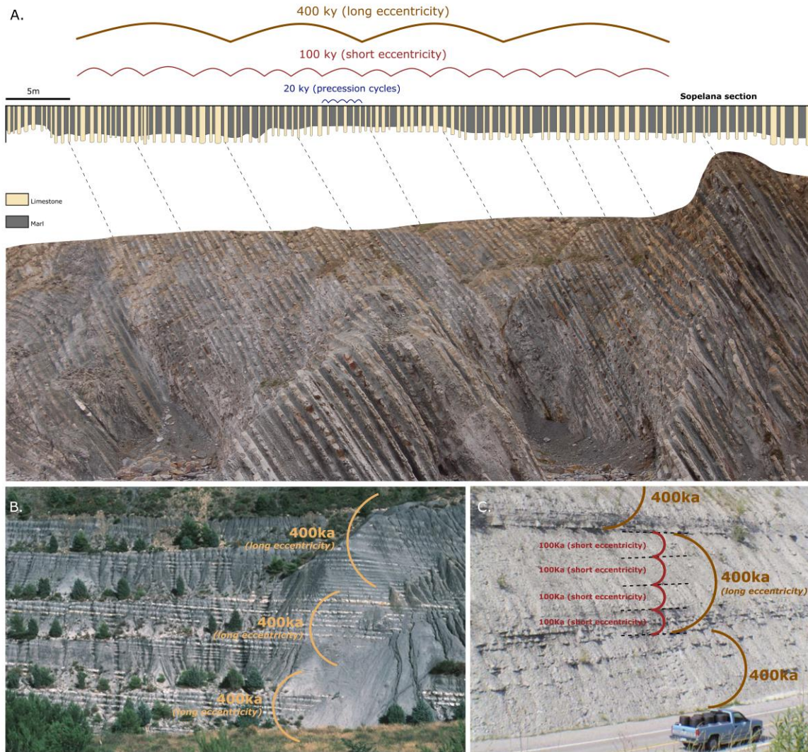
725 Figure 29. Outcrop examples of sedimentary cycles determined by cyclostratigraphic analysis: A – Long eccentricity, short eccentricity, and precession cycles in hemipelagic limestones and marls alternations of the Sopolana section (Maastrichtian), Spain (modified from Batenburg et al., 2014); B – Long eccentricity cycles in hemipelagic limestone and marl alternations of the La Marcouline section (Middle Aptian), France (modified from Kuhnt and Moullade, 2007); C – Long and short eccentricity cycles in shallow-marine deposits of the Kope Formation (Ordovician), United States (modified from Ellwood et al., 2013).
