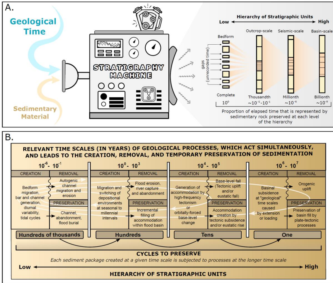
Figure 18. Stratigraphy Machine: A. Playful representation of the "Stratigraphy Machine" concept that generates the stratigraphic record, organizing geological time into hierarchically preserved sedimentary units and hiatus surfaces, from the bedform to the entire basin fill (based on Holbrook and Miall, 2020); B. Table illustrating the Stratigraphy Machine's operation, which considers the simultaneous action of several accumulation, removal, and preservation processes, which interact at different time scales to generate the rock record. For convenience, the time scale is subdivided into four broad intervals. The diagram should be read from left to right, where at each time interval the sediments are first generated by the depositional processes, and what is not removed on
