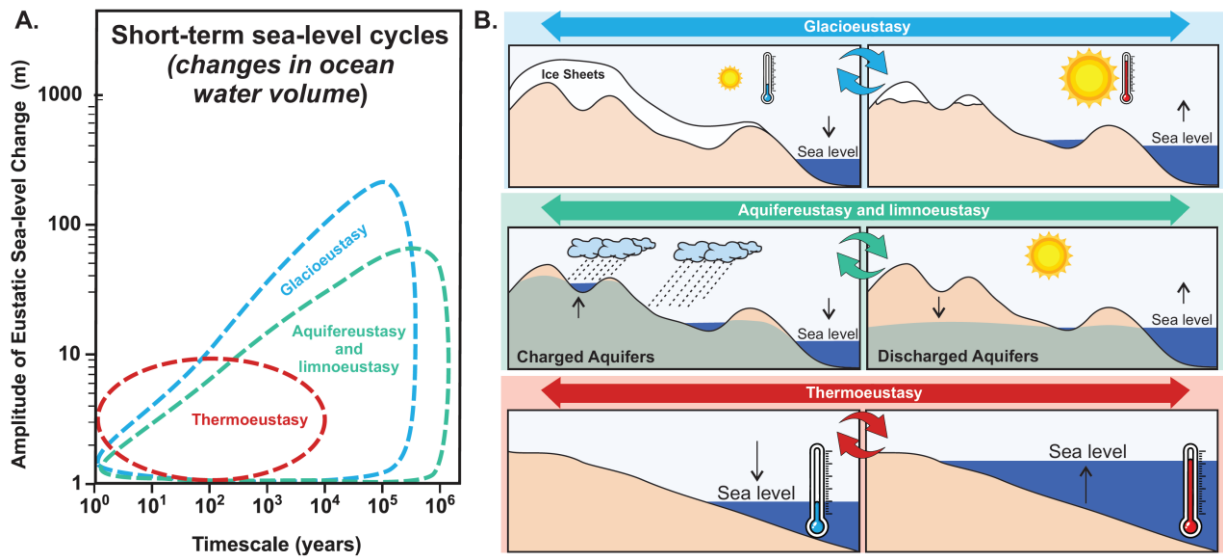
225 Figure 4. A - Log-scale diagram of the timing and amplitudes of the main mechanisms that control "short-term" sea-level variations. The values represented must be considered as averages (modified from Sames et al., 2016); B - Schematic diagrams representing the processes that promote changes in sea level (glacioeustasy, aquifereustasy + limnoeustasy, and thermoeustasy) during climate changes induced by orbital cycles.
