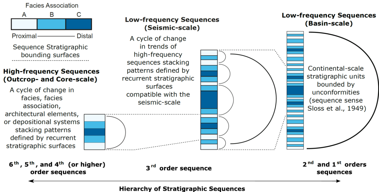
685 Figure 27. Hierarchical stratigraphic sequence framework (modified from Magalhães et al., 2020). High-frequency sequences (fourth or higher orders) are observed at outcrop- and core-scale. The vertical recurrence of high-frequency sequences composes the low-frequency sequences observed in seismic data (third-order). First- and second-order low-frequency sequences occur at basin-scale predominantly limited by unconformities, as proposed by Sloss et al. (1949).
