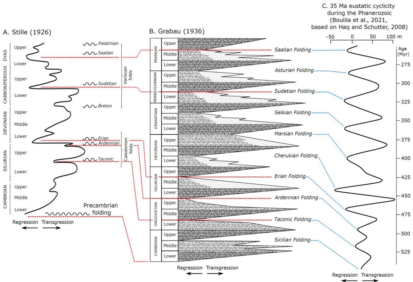
330 Figure 8. Global sea-level curves: A. Modified from Stille (1926) and B. modified from Grabau (1936). Both indicate the main orogenic periods associated with rapid marine regressions. The red lines indicate the same events identified by Stille (1926) and Grabau (1936). C. Paleozoic eustatic cycles of approximately 35 Myr (determined by bandpass filtering of data presented by Haq and Schutter, 2008) and potential correlation (blue lines) with equivalent cycles of Grabau (1936) (modified from Boulila et al., 2021).
