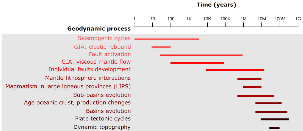
Figure 11. Temporal variability of the main periodic geodynamic mechanisms (based on Matenco and Haq, 2020).
