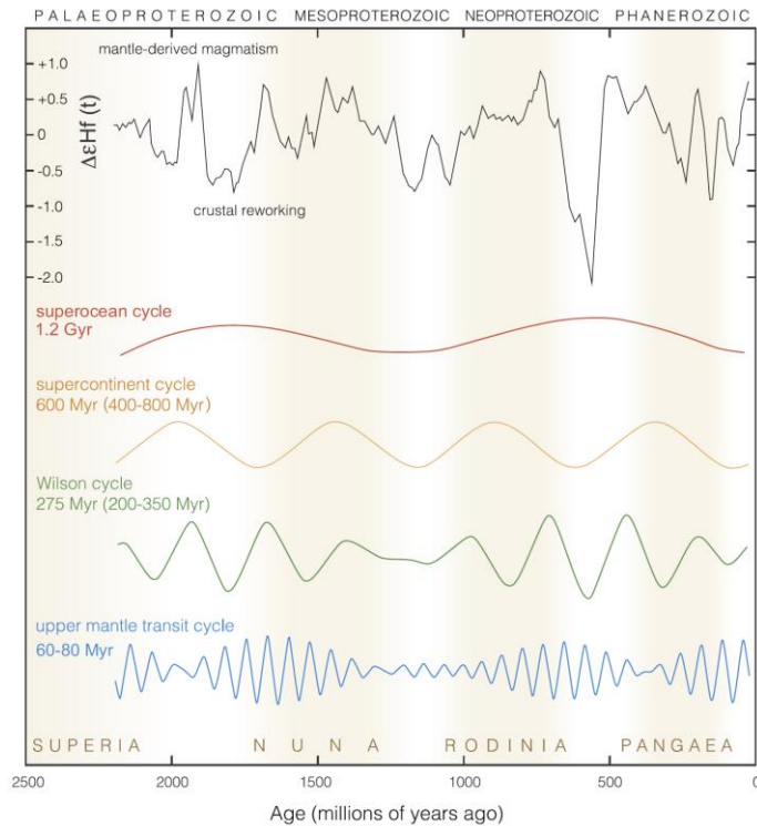
400 Figure 12. Global Hf database (black) and cycles determined by the time-series analysis: superocean cycle (~1.2 Gyr; red), the supercontinent cycle (~600 Myr; yellow), the Wilson cycle (~275 Myr; green), and an upper mantle cycle (~60–80 Myr; blue).
