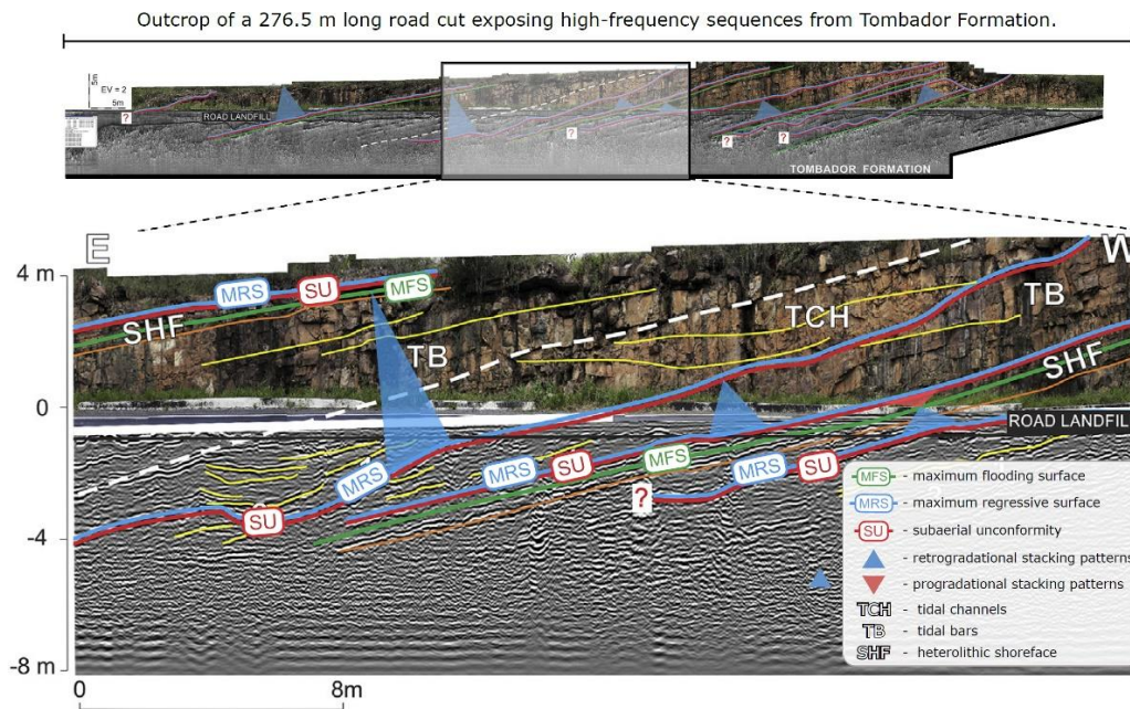
Figure 25. High-frequency sequences identified in an outcrop and in a GPR profile of the Tombador Formation (Mesoproterozoic), Chapada Diamantina Region, Brazil (modified from Magalhães et al., 2017). The sequences are composed of tidal channels and bars, bounded at the top by heterolithic intervals that configure cycles of retrogradational stacking patterns defined by the recurrence of the same type of stratigraphic surface in the geological record.
