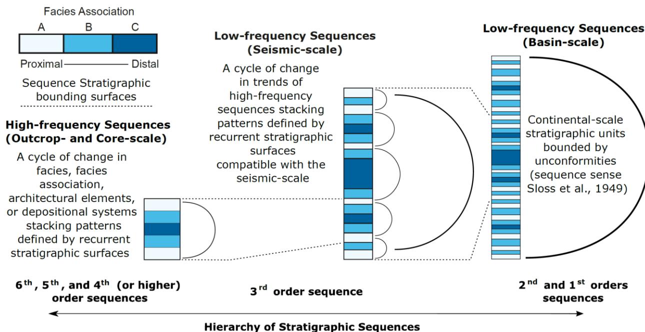
Figure 27. Hierarchical stratigraphic sequence framework (modified from Magalhães et al., 2020). High-frequency sequences (fourth or higher orders) are observed at outcrop- and core-scale. The vertical recurrence of high-frequency sequences composes the low-frequency sequences observed in seismic data (third-order). First- and second-order low-frequency sequences occur at basin-scale predominantly limited by unconformities, as proposed by Sloss et al. (1949).
