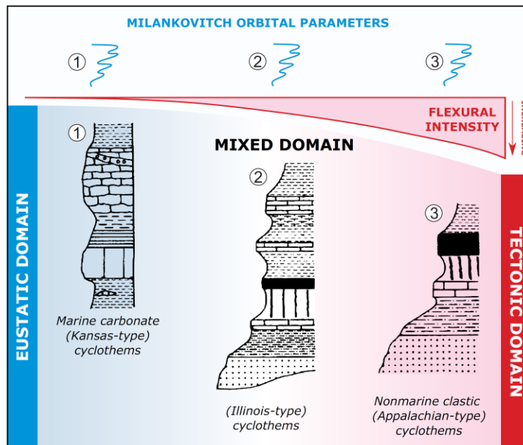
Figure 20. The genesis of the different types of cyclothem units in North America related to orbital parameters and lateral differences in the crust's flexural intensity (modified from Klein and Willard, 1989).
