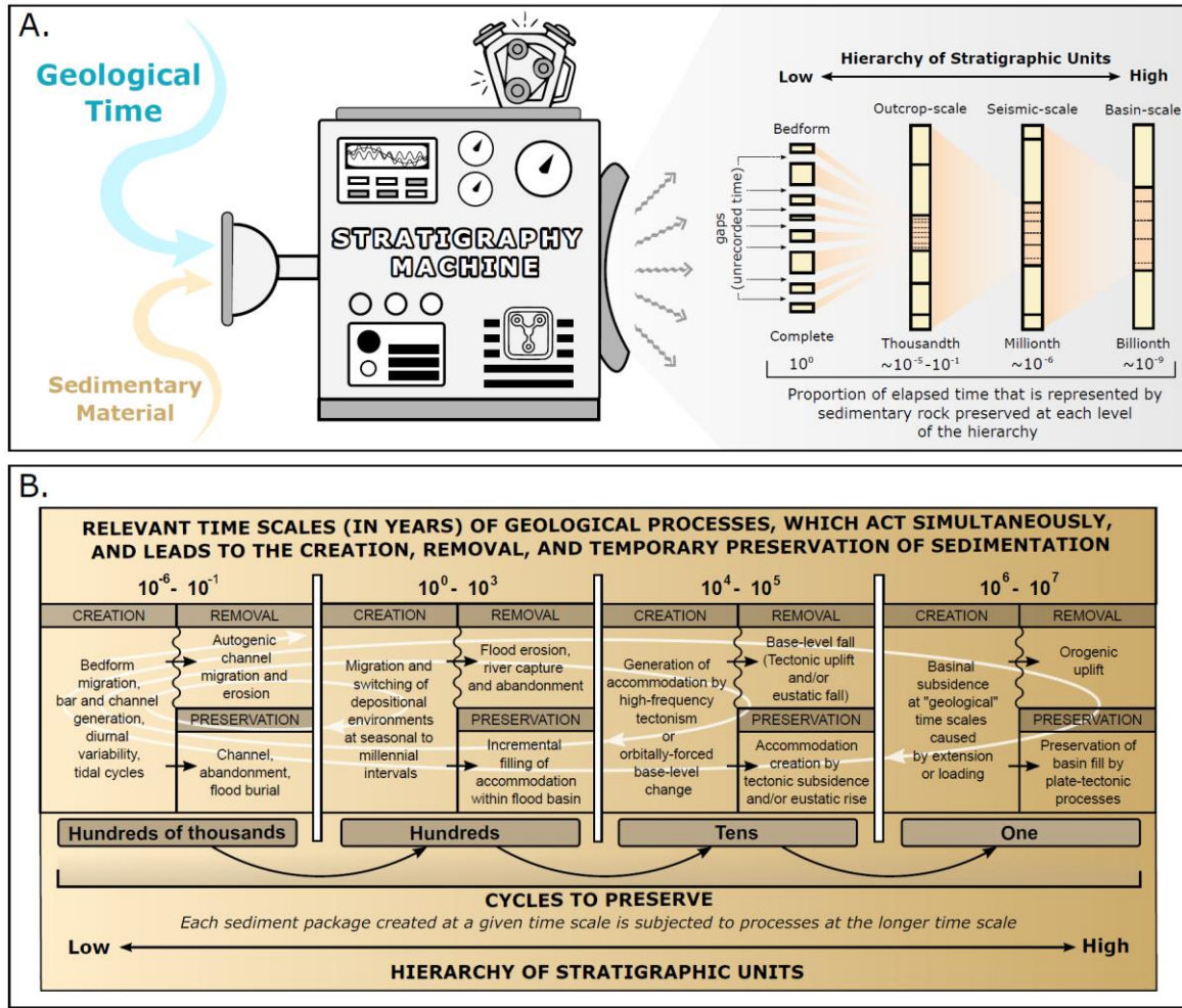
555 Figure 18. Stratigraphy Machine: A. Playful representation of the "Stratigraphy Machine" concept that generates the stratigraphic record, organizing geological time into hierarchically preserved sedimentary units and hiatus surfaces, from the bedform to the entire basin fill (based on Holbrook and Miall, 2020); B. Table illustrating the Stratigraphy Machine's operation, which considers the simultaneous action of several accumulation, removal, and preservation processes, which interact at different time scales to generate the rock record. For convenience, the time scale is subdivided into four broad intervals. The diagram should be read from left to right, where at each time interval the sediments are first generated by the depositional processes, and what is not removed on
