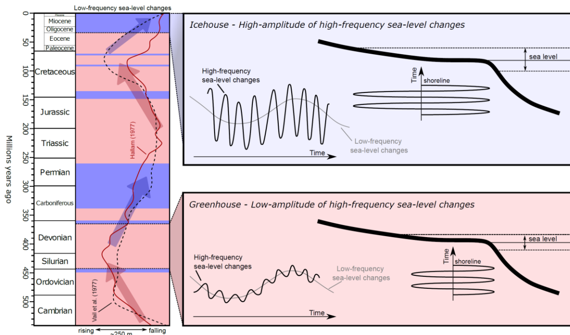
Figure 5. Changing frequencies and amplitudes of eustasy. Sea-level curves, according to Vail et al. (1977) and Hallam (1977). In icehouse periods, (in blue), these cycles have a high amplitude, mainly due to the effects of glacioeustasy. Eustatic oscillations have lower amplitude in greenhouse periods (in light red) since there is no significant glacial effect (modified from Wilson, 1998; Séranne, 1999; Montañez et al., 2011).
