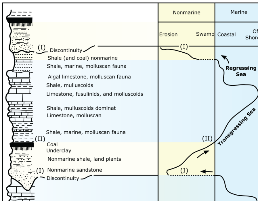
Figure 19. Representative section of cyclothem units indicating the alternation of continental and marine paleoenvironments (modified from Moore, 1964). The alternatives of limits for cyclothem units are: (I) disconformities; (II) the transition from non-marine to marine conditions.
