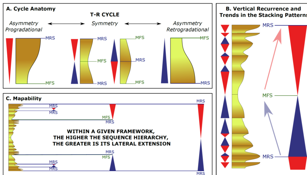
Figure 26. Characteristics and criteria for defining stratigraphic sequences within a cyclic and hierarchical framework (modified from Fragoso et al., 2021): A. T-R cycle anatomy. B. Vertical recurrence of individual cycles and trends in cyclic stacking pattern (modulation of the smallest by the highest hierarchy). C. Mappability of the stacking patterns and stratigraphic surfaces within a given framework, which is more significant the higher is the hierarchy. Abbreviations: MFS – maximum flooding surface; MRS – maximum regressive surface.
