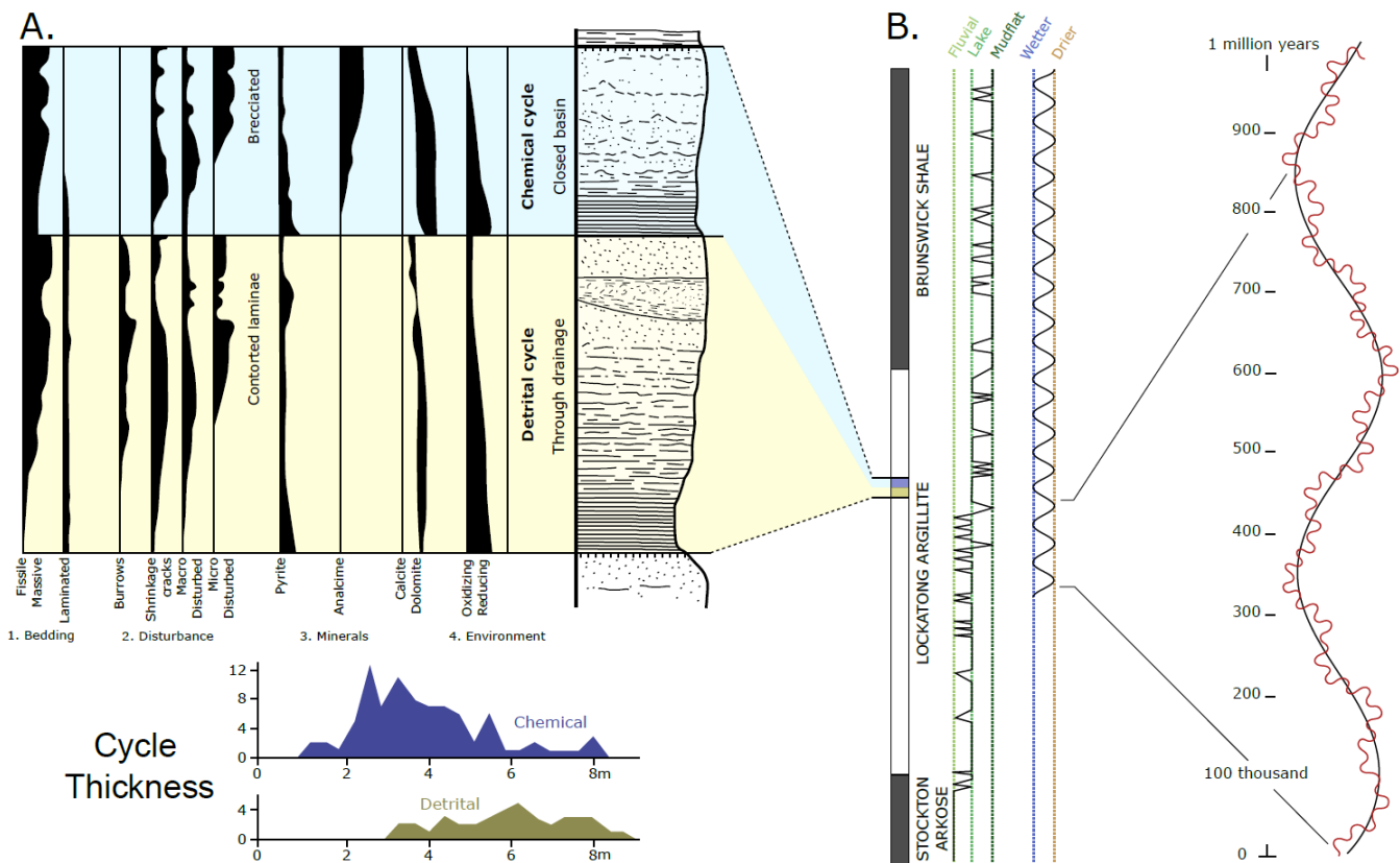
715 Figure 28. Cyclic lacustrine sedimentation of the Upper Triassic Lockatong Formation (modified from Van Houten, 1964): A. Model of detrital and chemical short cycles; B. Generalized stratigraphic section of Lockatong Formation and adjacent units. The columns show the alternating geographic environments and the long climatic cycles of wetter and drier phases. An age model is presented based on two long climatic cycles, with intermediate and short cycles associated.
