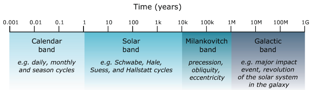
210 Figure 3. Logarithmic table of the astronomical cycle frequencies (adapted from House, 1995).
