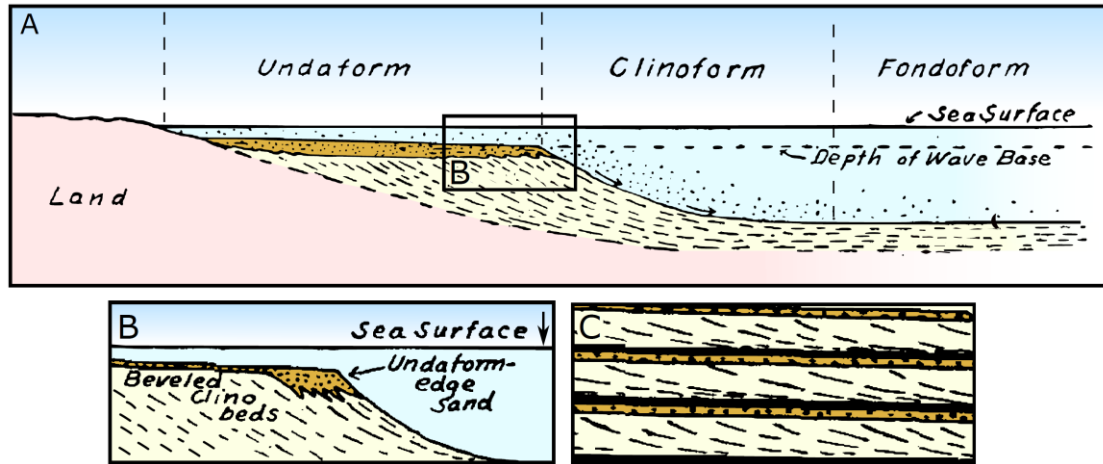
Figure 21. Sketches and terminology for coastal marine deposits (modified from Rich, 1951): A) Undaform, clinoform, fondoform; B) Area of thick sand on the outer edge produced by the slight reduction in sea level; C) Alternations of coastal marine deposits produced by intermittent changes in sea level.
