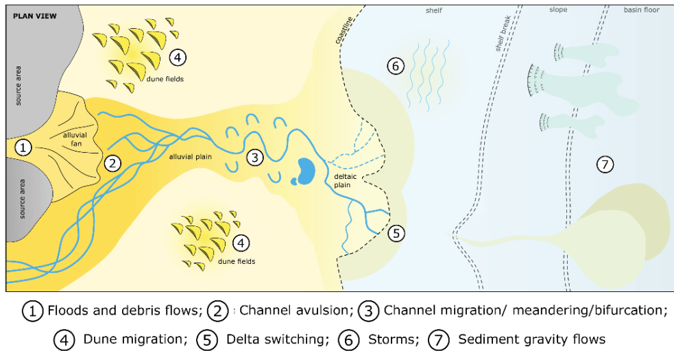
510 Figure 16. Schematic illustration with some autogenic controls on sedimentation in different environments.
