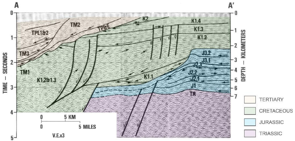
Figure 24. Seismic section from offshore northwest Africa showing sequences defined by seismic reflectors. Black lines show the sequence boundaries (modified from Mitchum and Vial, 1977).
