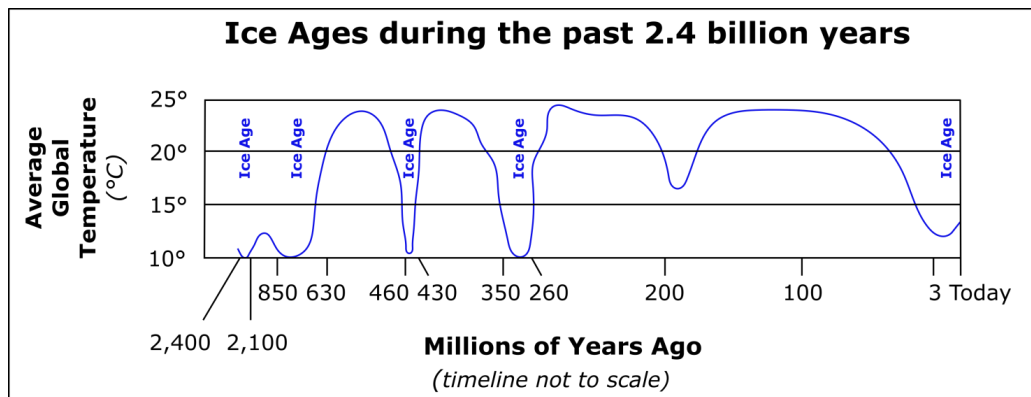
710 Figure 1: The chart shows five major ice ages during the past 2.4 billion years. Adapted from Utah Geological Survey Notes, Eldredge S. and Biek B. (2010) [Adapted from Saltzman (2002)], Retrieved from https://geology.utah.gov/wp-content/uploads/ice_ages1 . © Copyright –Utah Geological Survey– State of Utah. May, 15, 2017.
