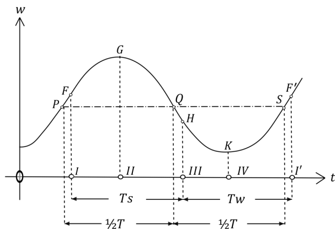
750 Figure 5: The annual march of the irradiation for any arbitrary latitude. Reprinted from Kanon der Erdbestrahlung und seine Anwendung auf das Eiszeitenproblem (p.272) by Milankovitch, M., 1941, Belgrade: Royal Serbian Academy Special Publications.
