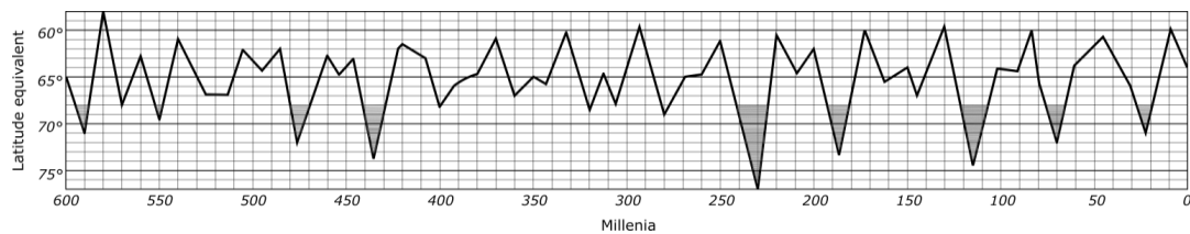
755 Figure 6: The equivalent graph which shows the variations of the summer insolation for 65° N. Reprinted from Kanon der Erdbestrahlung und seine Anwendung auf das Eiszeitenproblem (p.415) by Milankovitch, M., 1941, Belgrade: Royal Serbian Academy Special Publications.
