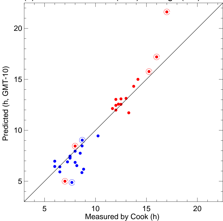
(a) Tahiti times of low (blue) and high (red) waters
