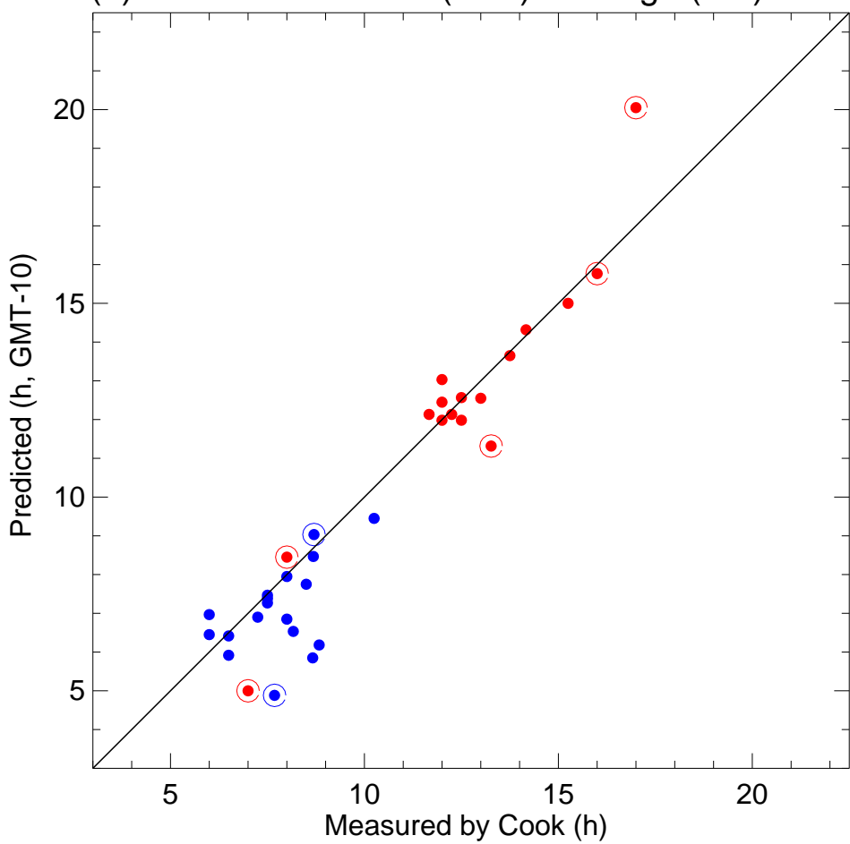
(b) Tahiti times of low (blue) and high (red) waters
