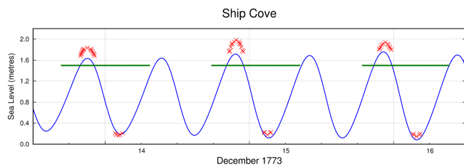
Figure 11. Sea level observations made by William Bayly at Ship Cove during December 1773 plotted with a predicted tidal curve based on modern data and with lines indicating when the Moon was above the horizon.
