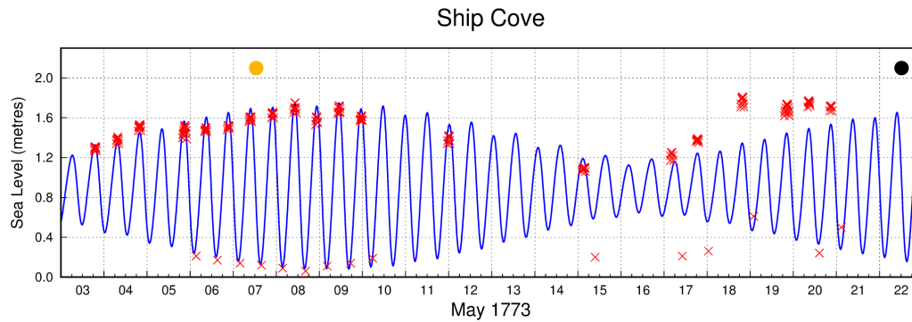
Figure 7. Sea level observations made by William Bayly at Ship Cove during May 1773 plotted with a predicted tidal curve based on modern data.
