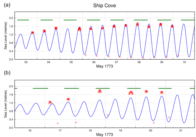
Figure 12. Sea level observations made by William Bayly at Ship Cove during May 1773 plotted with a predicted tidal curve based on modern data and with lines indicating when the Moon was above the horizon.
