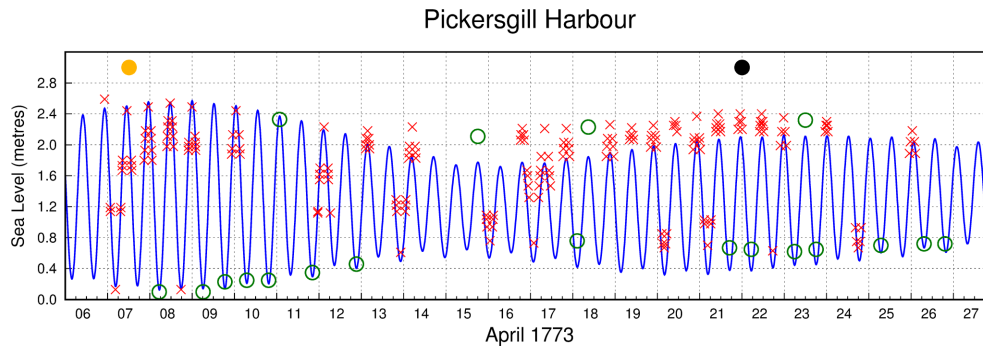
Figure 5. Sea level observations made by William Wales at Pickersgill Harbour during April 1773 plotted with a predicted tidal curve based on modern data.
