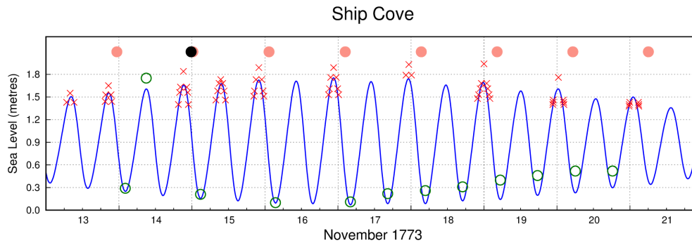
Figure 8. Sea level observations made by William Wales at Ship Cove during November 1773 plotted with a predicted tidal curve based on modern data. Salmon-coloured dots indicate the time of lunar transit; dates and times of lunar transit, as calculated using Gray (2020), are given in Table C3 in Appendix C; and the black dot is new Moon.
