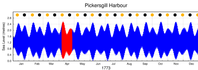
Figure 6. The predicted tide curve throughout 1773 at Pickersgill Harbour; the portion in red corresponds to the period when Wales was making his observations.
